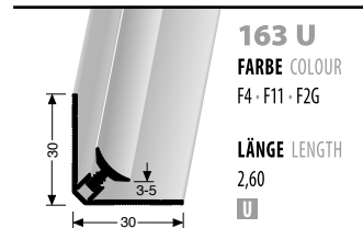
2-TEILIGE CLIP-INNENECKE 2-PART CLIP INTERIOR CORNER
